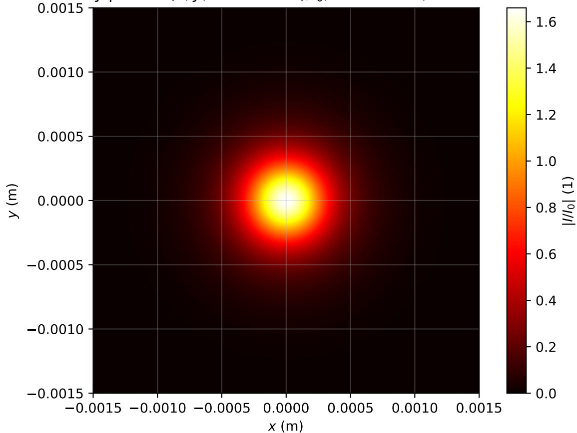
Intensity profile I(x, y, z = 1.194m)/I_0 , Pin=1.0Pcr, artificial time
